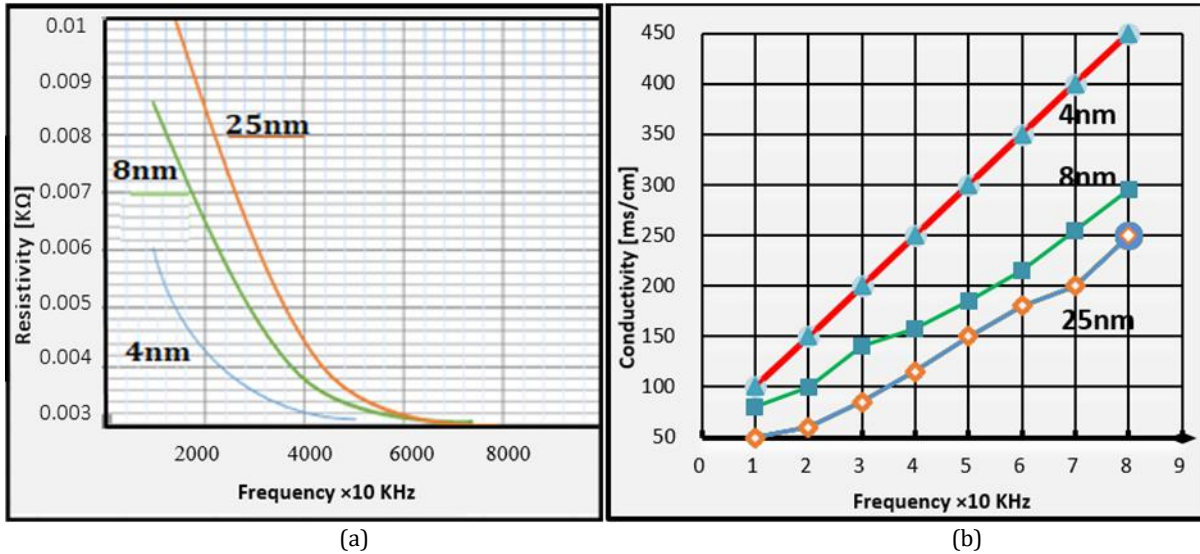
Figure 8. Characterization for different sizes of fabricated nano gap structures: (a) Resistivity, (b) Conductivity.
