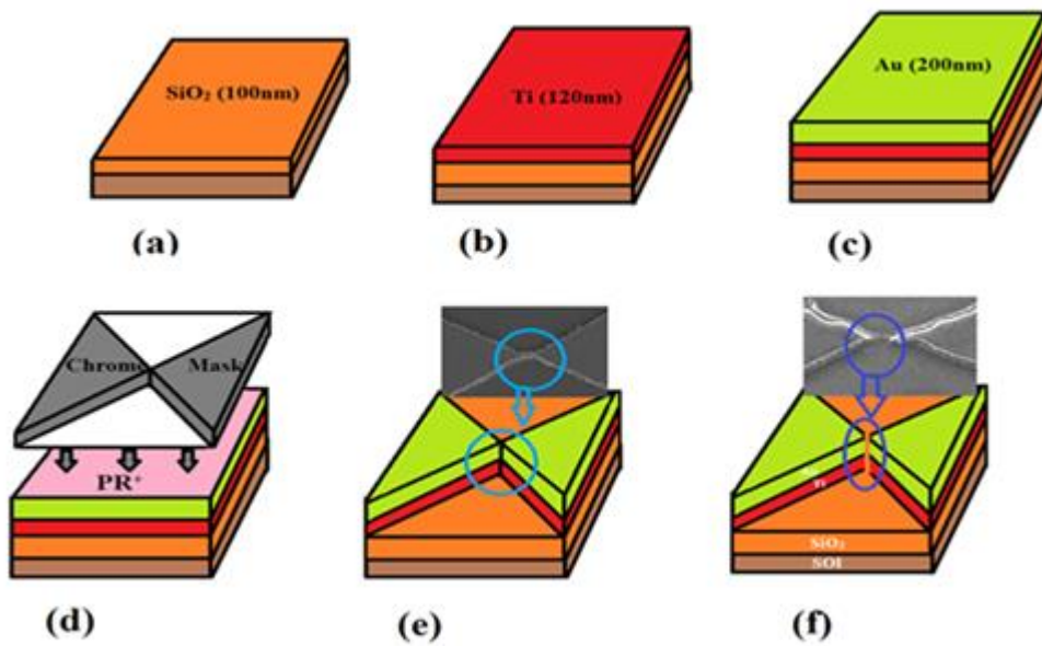
Figure 2. Cross-sectional view of the proposed fabrication process flow of Au/Ti nano gap structure: (a) deposition of 100nm SiO 2 layer, (b) Ti deposition layers, (c) Au 200nm deposition layer, (d) chrome mask exposure and photoresist removing from Au/Ti structure, (e) uncovered area remain intact with zero gap dimension, and (f) gold nano gaps after aqua regia wet etching.
