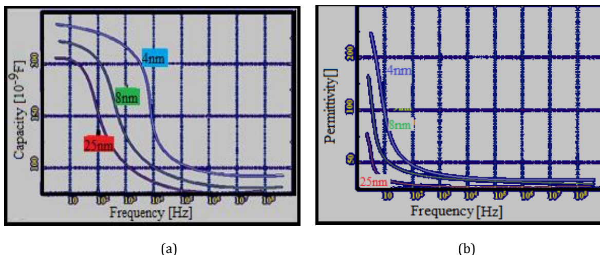
Figure 7. (a) Capacitance-Frequency, and (b) Permittivity-frequency analysis for the fabricated three sizes of nano gap.
